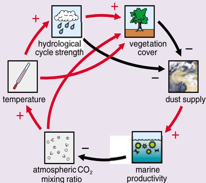
Figure. Some of the potential feedbacks involving dust and iron fertilisation in the climate system. Positively correlated connections are shown in red, and negative ones in black. Four main (positive) feedback loops exist in this system, each having a total of two negatively correlated connections within the loop;
