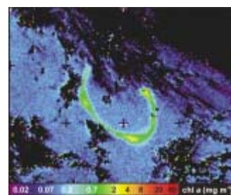
Figure 1. Ocean colour satellite (SeaWiFS) image of concentrations of surface ocean chlorophyll (a phytoplankton photosynthetic pigment, whose concentration can be taken as a rough indicator of cell density), taken some 6 weeks after the deliberate release of iron in the Southern Ocean [1]. The contrast between the 'fertilised' area (green/yellow colour) and the surrounding ('unfertilised') waters (blue) can be clearly made out (note: black pixels in the image represent cloud cover). (SeaWiFS data provided by the NASA DAAC/GSFC and copyright of Orbital Imaging Corps and the NASA SeaWiFS project, and processed at CCMS-PML.)
